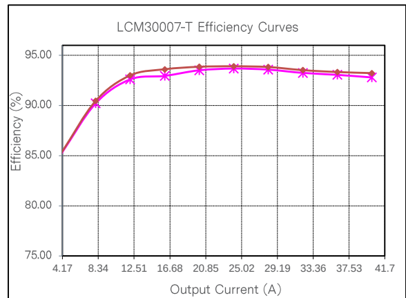
Figure 82: LCM30007-T Efficiency Curve @ 25°C Loading: I_{o\_main} = 10\% I_{o\_max} increment to 41.7A, I_{sb} = 0A
