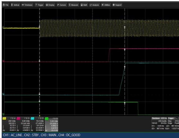
Figure 43: LCM3000U-T Turn-on delay via AC mains
