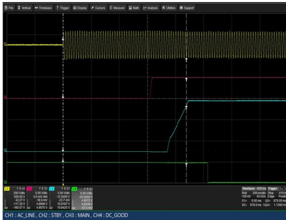
Figure 1: LCM3000L-T Turn-on delay via AC mains Vin = 90VAC Load: Io = 125A (12V), Isb = 2A Ch 1: Vin Ch 2: Vsb Ch 3: Vo Ch 4: G_DCOK_C
