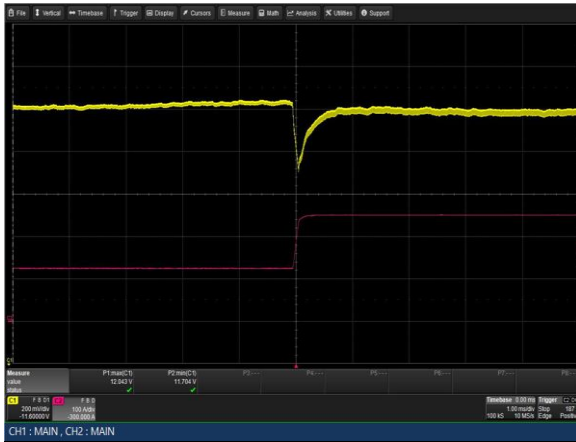
Figure 9: LCM3000L-T Transient Response - V_o Deviation 50% to 100% load change 1A/uS slew rate V_{in} = 230VAC Ch 1: V_o Ch 2: I_o
