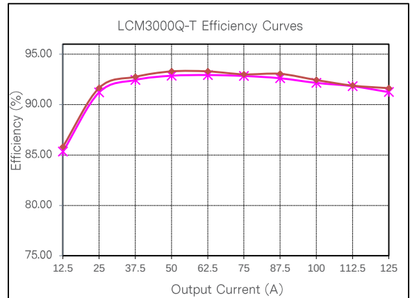
Figure 40: LCM3000Q-T Efficiency Curve @ 25°C Loading: I_{o\_main} = 10\% I_{o\_max} increment to 125A, I_{SB} = 0A —x— 230VAC —◆— 264VAC
