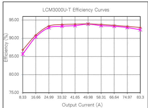
Figure 54: LCM3000U-T Efficiency Curve @ 25°C Loading: Io_main = 10%Io_max increment to 83.3A, Isb = 0A
