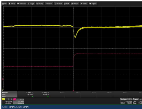
Figure 65: LCM3000W-T Transient Response - V_o Deviation 50% to 100% load change 1A/uS slew rate V_{in} = 230VAC Ch 1: V_o Ch 2: I_o
