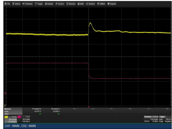
Figure 38: LCM3000Q-T Transient Response - V_o Deviation 100% to 50% load change 1A/uS slew rate V_{in} = 230VAC Ch 1: V_o Ch 2: I_o
