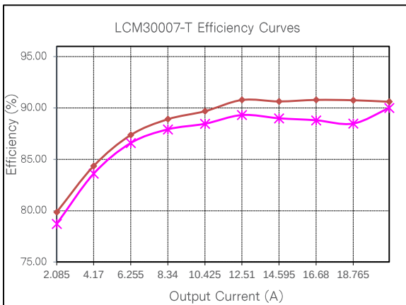
Figure 81: LCM30007-T Efficiency Curve @ 25°C Loading: I_{o\_main} = 10\% I_{o\_max} increment to 20.8A, I_{sb} = 0A
