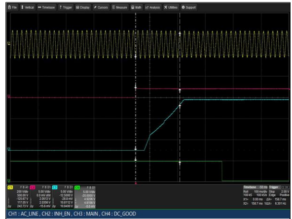
Figure 2: LCM3000L-T Turn-on delay via INH_EN Vin = 90VAC Load: Io = 125A (12V), Isb = 2A Ch 1: Vin Ch 2: INH_EN Ch 3: Vo Ch 4: G_DCOK_C
