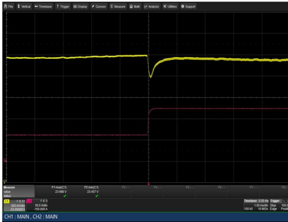
Figure 37: LCM3000Q-T Transient Response - V_o Deviation 50% to 100% load change 1A/uS slew rate V_{in} = 230VAC Ch 1: V_o Ch 2: I_o
