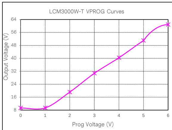
Figure 69: LCM3000W-T Output Voltage Adjustment by VPROG @ 25°C * 115VAC Loading: I_o = 0A (48V), I_{sb} = 0A
