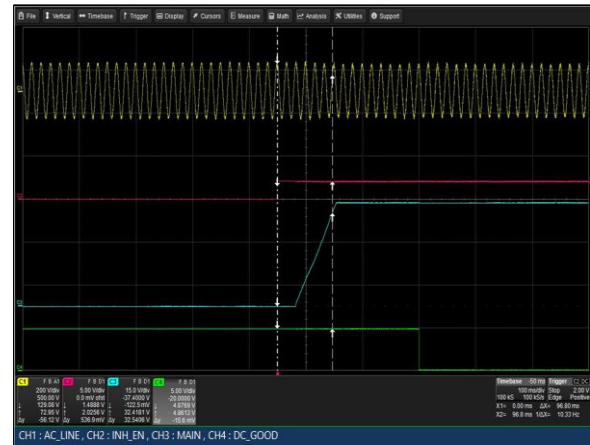
Figure 44: LCM3000U-T Turn-on delay via INH_EN
