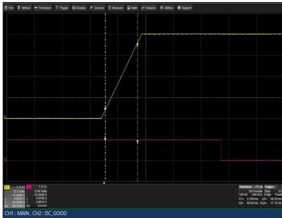
Figure 63: LCM3000W-T Output Voltage Startup V_{in} = 264VAC Load: I_o = 62.5A ( 48V ), I_{sb} = 2A Ch 1: V_o Ch 2: G\_DCOK\_C
