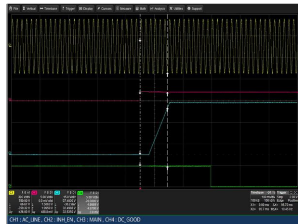
Figure 46: LCM3000U-T Turn-on delay via INH_EN
