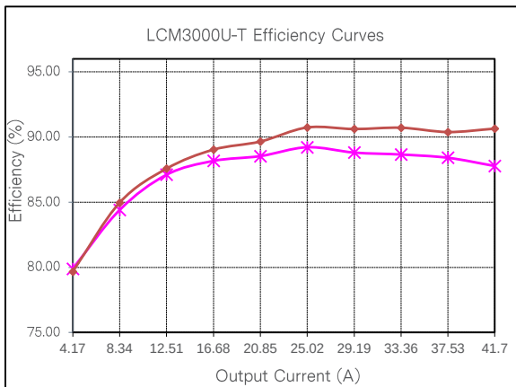
Figure 53: LCM3000U-T Efficiency Curve @ 25°C Loading: Io_main = 10%Io_max increment to 41.7A, Isb = 0A
