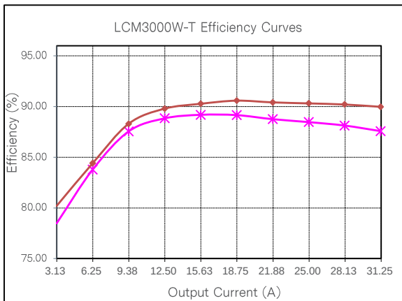
Figure 67: LCM3000W-T Efficiency Curve @ 25°C Loading: I_{o\_main} = 10\% I_{o\_max} increment to 31.25A, I_{sb} = 0A
