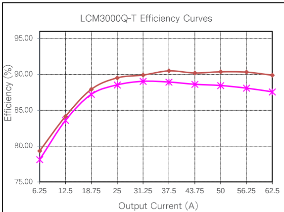
Figure 39: LCM3000Q-T Efficiency Curve @ 25°C Loading: I_{o\_main} = 10\% I_{o\_max} increment to 62.5A, I_{SB} = 0A —x— 90VAC —◆— 115VAC
