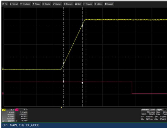
Figure 7: LCM3000L-T Output Voltage Startup V_{in} = 264VAC Load: I_o = 125A ( 12V ), I_{sb} = 2A Ch 1: V_o Ch 2: G\_DCOK\_C
