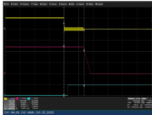
Figure 64: LCM3000W-T Turn Off Characteristic via INH_EN V_{in} = 264VAC Load: I_o = 62.5A ( 48V ), I_{sb} = 2A Ch 1: INH_EN Ch 2: V_o Ch 3: G\_DCOK\_C
