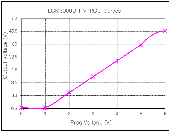
Figure 55: LCM3000U-T Output Voltage Adjustment by VPROG @ 25°C * 115VAC Loading: I_o = 0A (36V), I_{sb} = 0A
