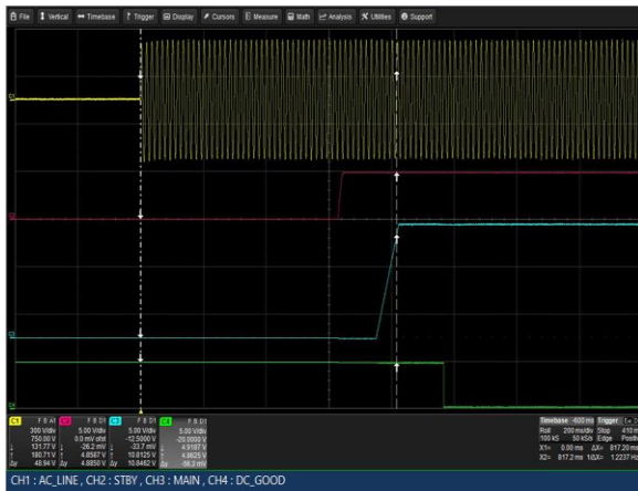
Figure 3: LCM3000L-T Turn-on delay via AC mains Vin = 264VAC Load: Io = 250A (12V), Isb = 2A Ch 1: Vin Ch 2: Vsb Ch 3: Vo Ch 4: G_DCOK_C
