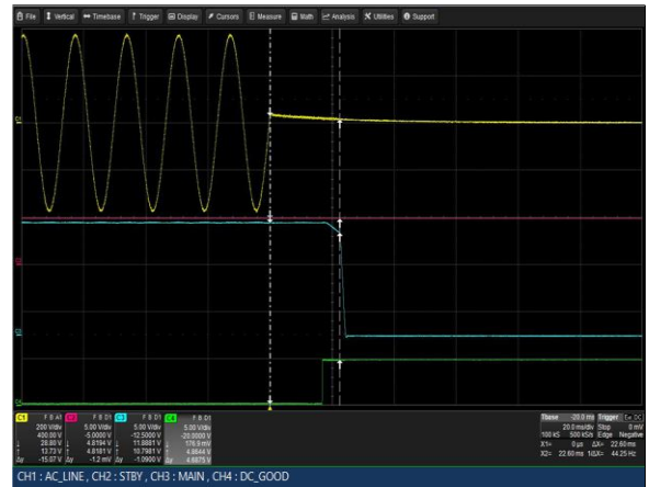
Figure 6: LCM3000L-T Hold-up Time Vin = 264VAC Load: Io = 250A (12V), Isb = 2A Ch 1: Vin Ch 2: Vsb Ch 3: Vo Ch 4: G_DCOK_C
