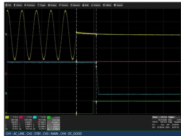
Figure 48: LCM3000U-T Hold-up Time
