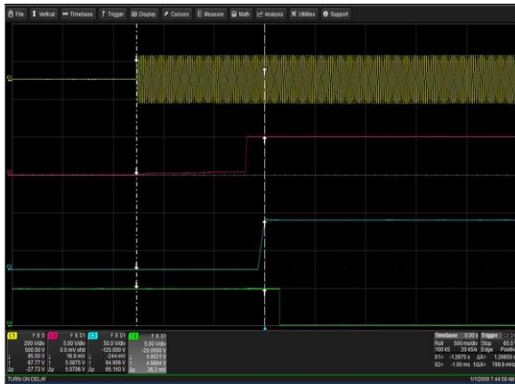
Figure 71: LCM30007-T Turn-on delay via AC mains
