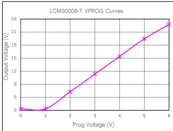
Figure 27: LCM30008-T Output Voltage Adjustment by VPROG @ 25°C * 115VAC Loading: I_o = 0A (18V), I_{sb} = 0A
