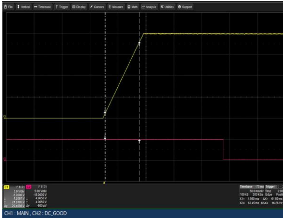
Figure 35: LCM3000Q-T Output Voltage Startup V_{in} = 264VAC Load: I_o = 125A (24V), I_{SB} = 2A Ch 1: V_o Ch 2: G\_DCOK\_C
