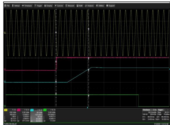
Figure 74: LCM30007-T Turn-on delay via INH_EN
