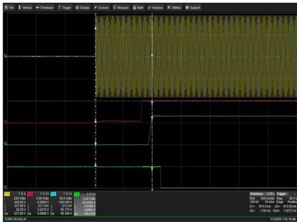
Figure 73: LCM30007-T Turn-on delay via AC mains
