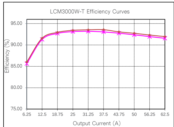
Figure 68: LCM3000W-T Efficiency Curve @ 25°C Loading: I_{o\_main} = 10\% I_{o\_max} increment to 62.5A, I_{sb} = 0A
