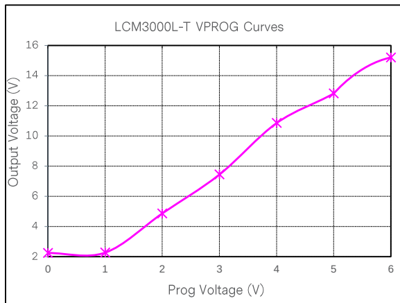
Figure 13: LCM3000L-T Output Voltage Adjustment by VPROG @ 25°C * 115VAC Loading: I_o = 0A (12V), I_{SB} = 0A
