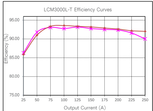
Figure 12: LCM3000L-T Efficiency Curve @ 25^{\circ}C Loading: I_{o,main} = 10\% I_{o,max} increment to 250A, I_{sb} = 0A
