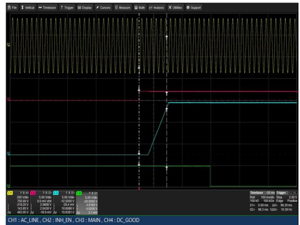
Figure 4: LCM3000L-T Turn-on delay via INH_EN Vin = 264VAC Load: Io = 250A (12V), Isb = 2A Ch 1: Vin Ch 2: INH_EN Ch 3: Vo Ch 4: G_DCOK_C
