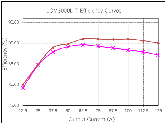
Figure 11: LCM3000L-T Efficiency Curve @ 25^{\circ}C Loading: I_{o,main} = 10\% I_{o,max} increment to 125A, I_{sb} = 0A
