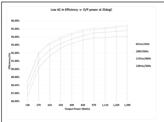
Figure 11: AIF06ZPFC Efficiency Curve @ 25°C — 85VAC — 100VAC — 115VAC — 120VAC Loading: P_{O,max} = 1400W 10% increment to P_{O,max}
